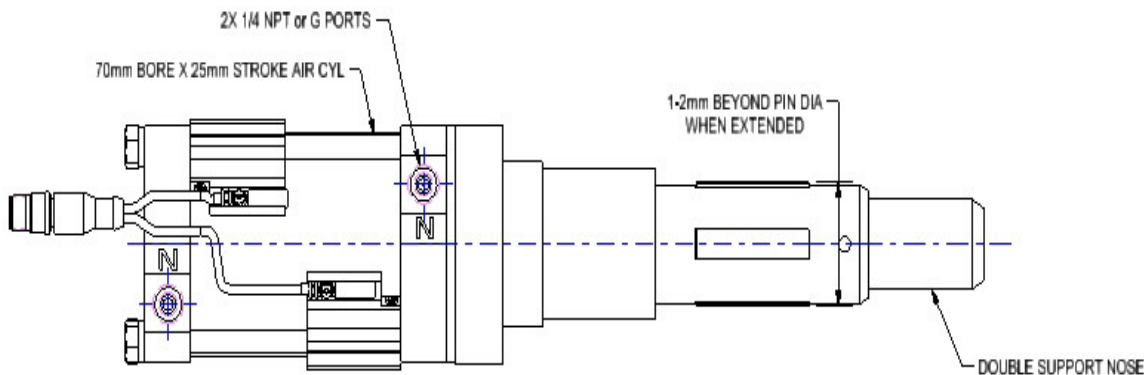
VIEW SHOWN WITH FINGERS EXTENDED
