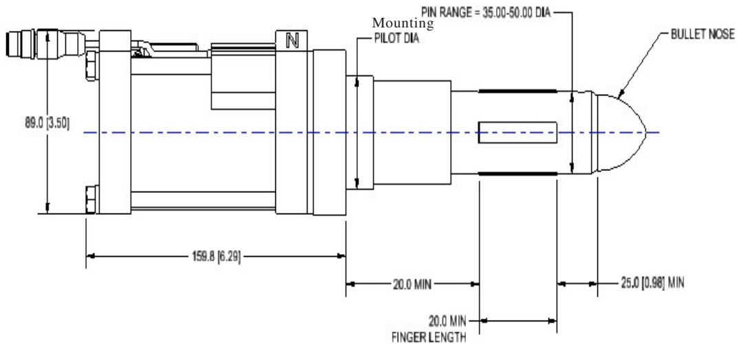
VIEW SHOWN WITH FINGERS EXTENDED
