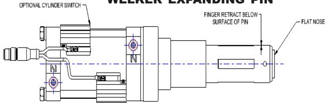
VIEW SHOWN WITH FINGERS RETRACTED
